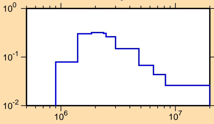
\sigma vs. E for ^{51}\text{Cr}(n,n_3)
