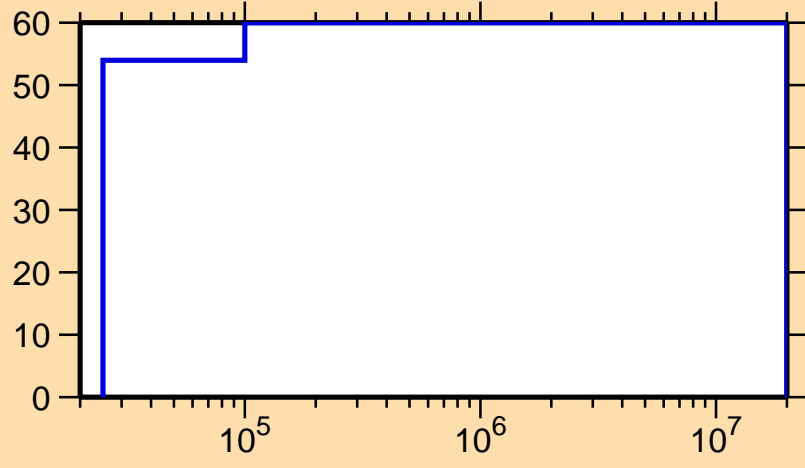
\Delta\sigma/\sigma vs. E for ^{51}\text{Cr}(n,\gamma)
