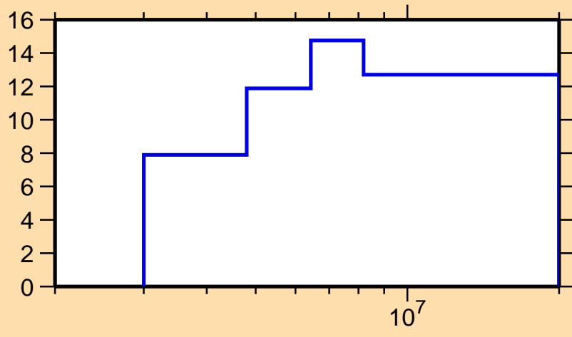
\Delta\sigma/\sigma vs. E for ^{51}\text{Cr}(n,el.)
