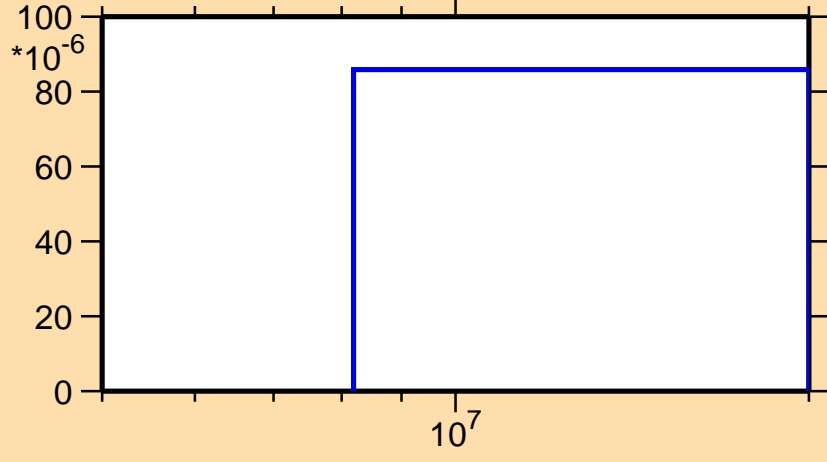
\sigma vs. E for ^{51}\text{Cr}(n,t)
