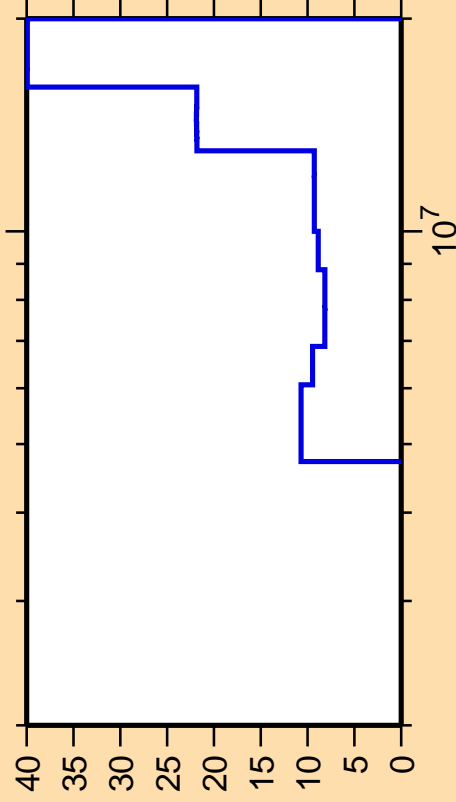
\Delta\sigma/\sigma vs. E for ^{52}\text{Cr}(n,\text{ncont.})
