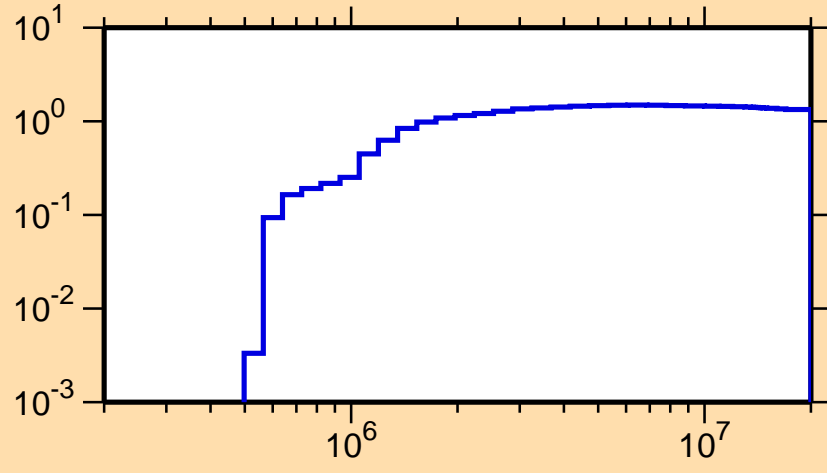
\sigma vs. E for ^{53}\text{Cr}(n,\text{nonel.})
