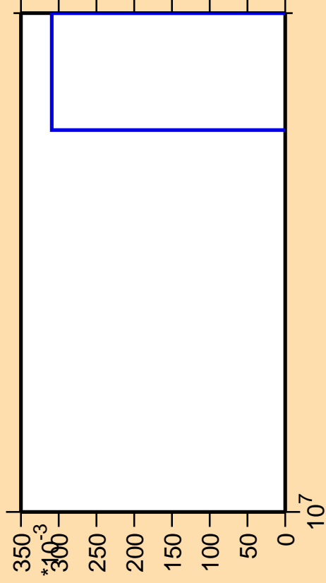
\Delta\sigma/\sigma vs. E for ^{53}\text{Cr}(n,2n\alpha)
