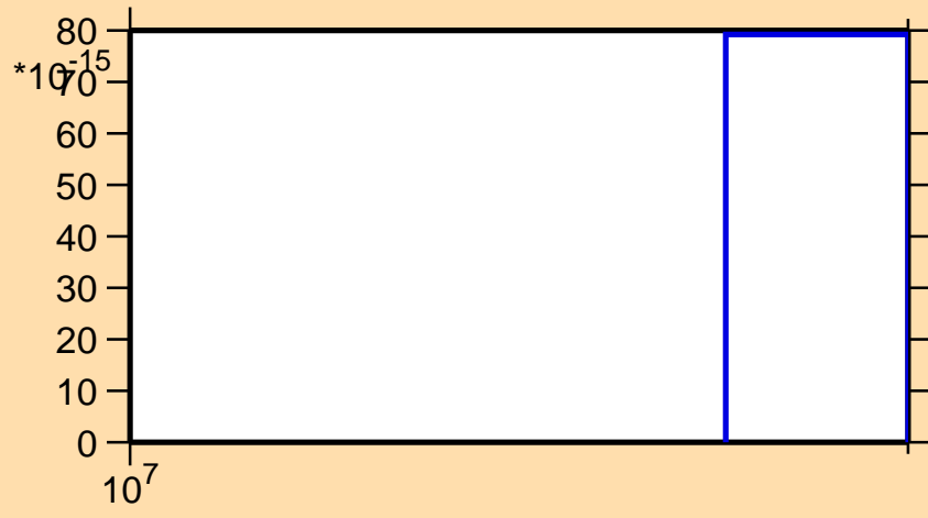
\sigma vs. E for ^{53}\text{Cr}(n,2n\alpha)
