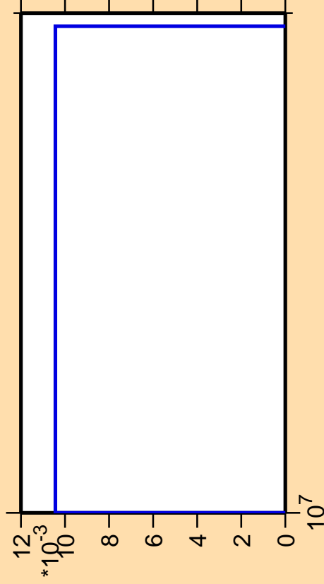
\Delta\sigma/\sigma vs. E for ^{54}\text{Cr}(n,p\alpha)
