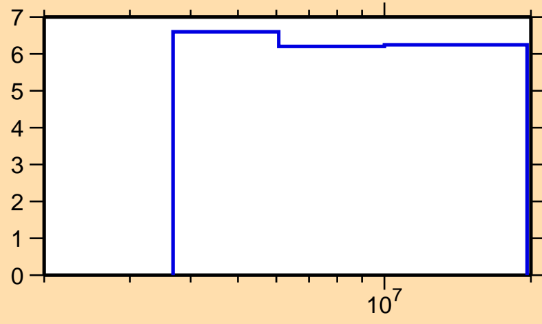
\Delta\sigma/\sigma vs. E for ^{54}\text{Cr}(n,n\text{onel.})
