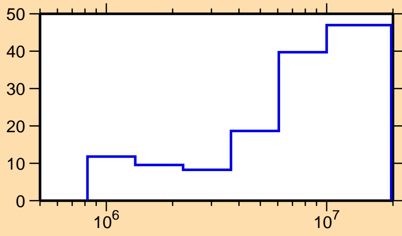
\Delta\sigma/\sigma vs. E for ^{54}\text{Cr}(n,n_1)
