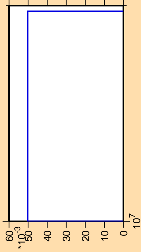
\Delta\sigma/\sigma vs. E for ^{54}\text{Cr}(n,\text{nd})
