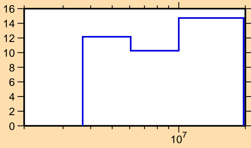
\Delta\sigma/\sigma vs. E for ^{54}\text{Cr}(n,n\text{cont.})
