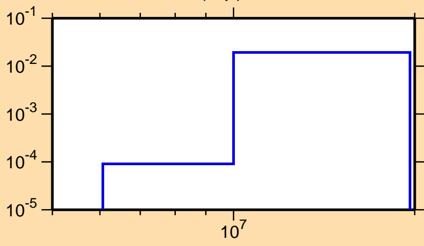
\sigma vs. E for ^{54}\text{Cr}(n,p)
