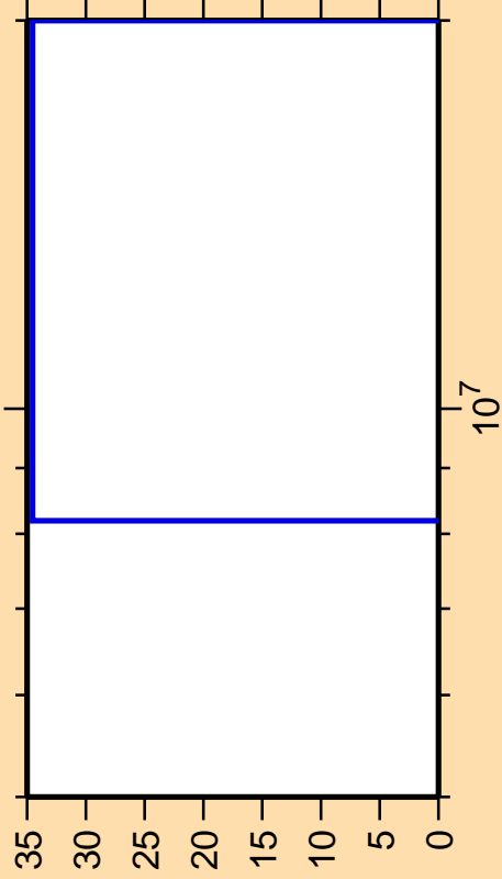
\Delta\sigma/\sigma vs. E for ^{54}\text{Cr}(n,n\alpha)
