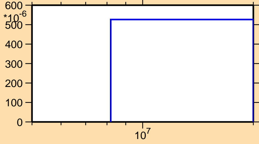
\sigma vs. E for ^{54}\text{Cr}(n,n\alpha)
