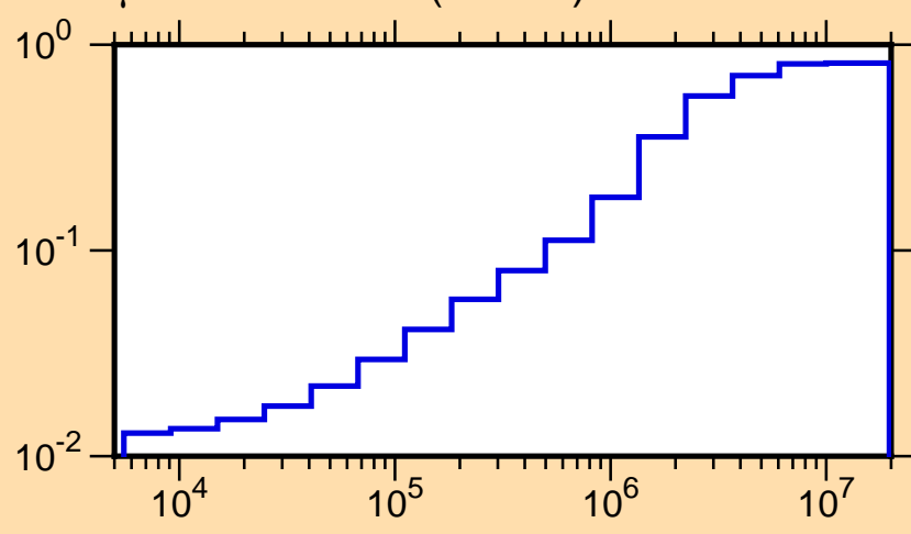
\mu vs. E for ^{55}\text{Cr}(\text{mt251})
