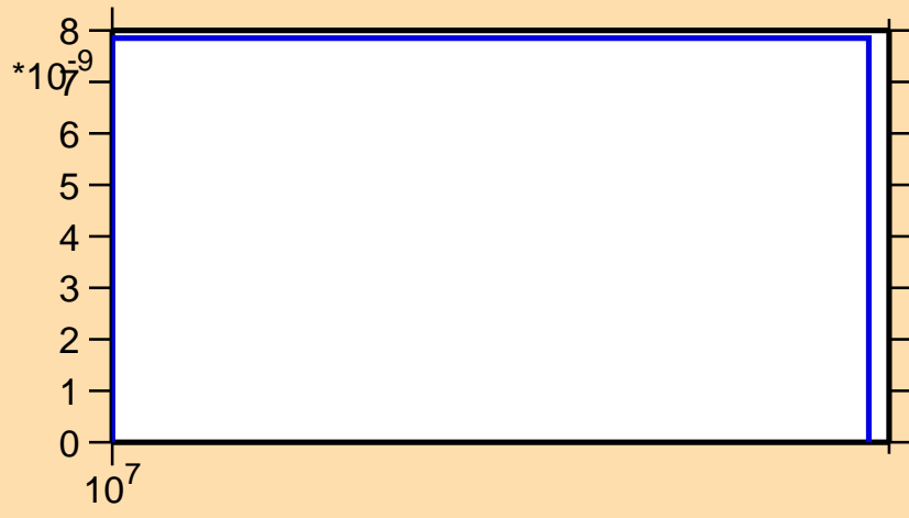
\sigma vs. E for ^{55}\text{Cr}(n,nd)
