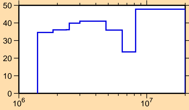
\Delta\sigma/\sigma vs. E for ^{55}\text{Cr}(n,\gamma)
