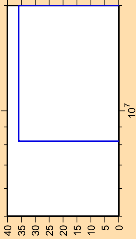
\Delta\sigma/\sigma vs. E for ^{55}\text{Cr}(n,n\alpha)
