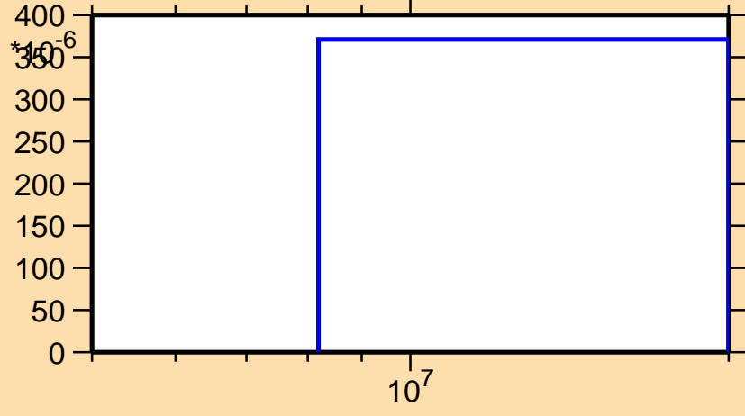
\sigma vs. E for ^{55}\text{Cr}(n,n\alpha)
