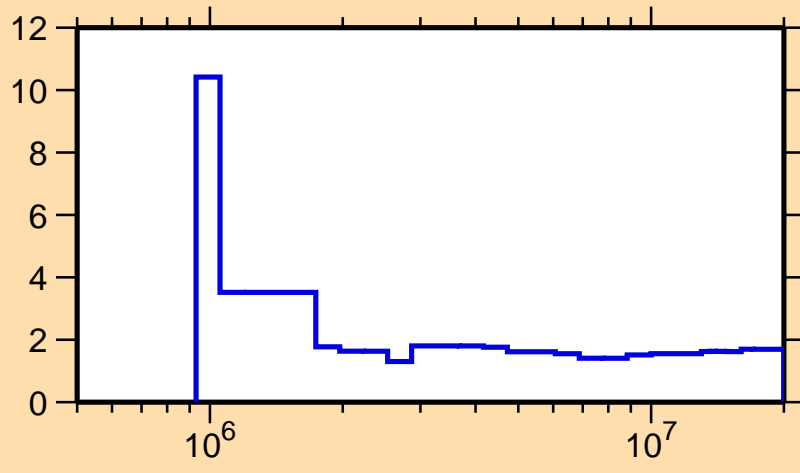
\Delta\sigma/\sigma vs. E for ^{56}\text{Cr}(n,\text{nonel.})
