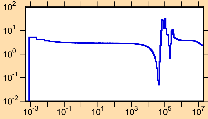
\sigma vs. E for ^{56}\text{Cr}(n,\text{tot.})
