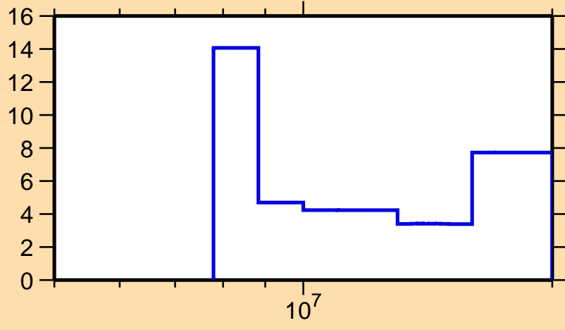
\Delta\sigma/\sigma vs. E for ^{56}\text{Cr}(n,2n)
