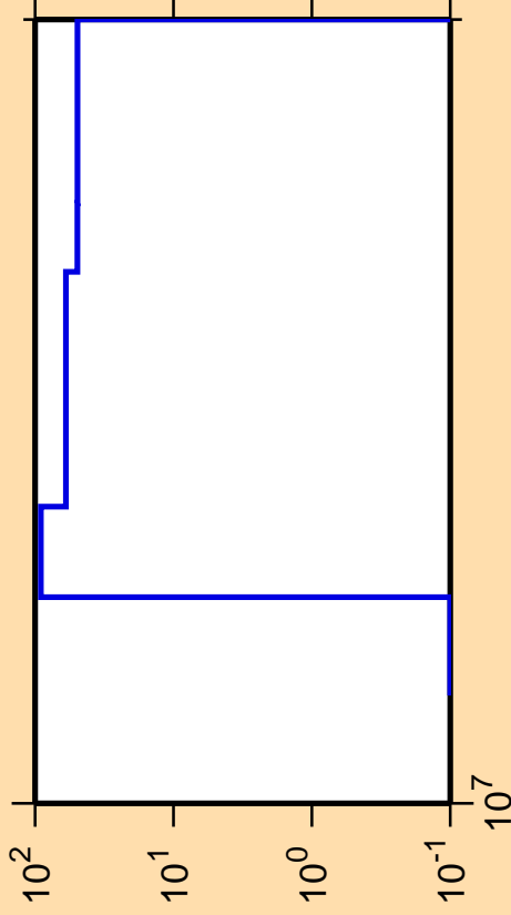
\Delta\sigma/\sigma vs. E for ^{56}\text{Cr}(n,d)
