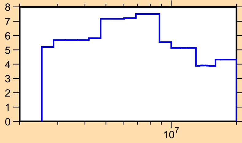
\Delta\sigma/\sigma vs. E for ^{57}\text{Cr}(n,\text{tot.})
