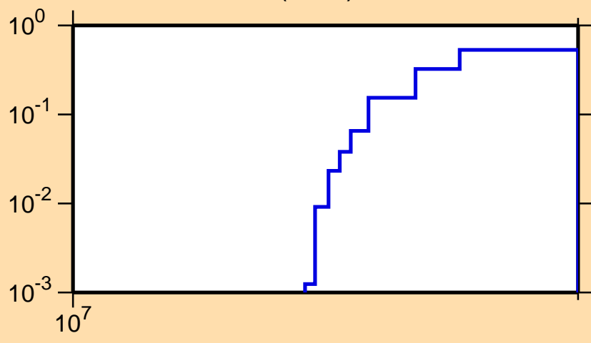
\sigma vs. E for ^{57}\text{Cr}(n,3n)
