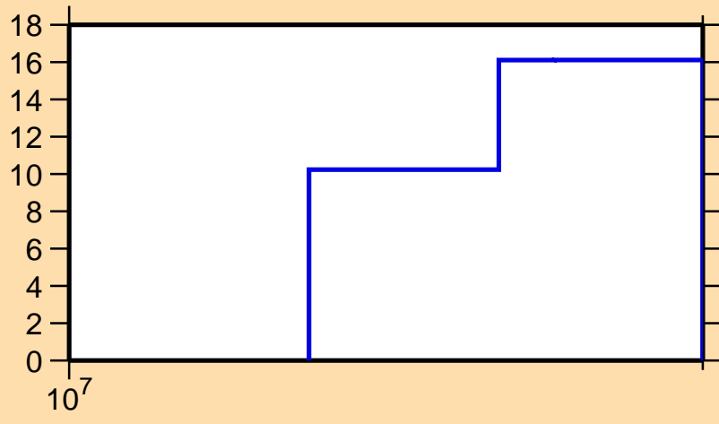
\Delta\sigma/\sigma vs. E for ^{57}\text{Cr}(n,2n)
