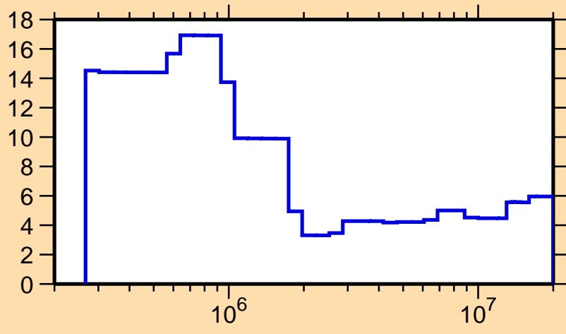
\Delta\sigma/\sigma vs. E for ^{57}\text{Cr}(n,\text{nonel.})
