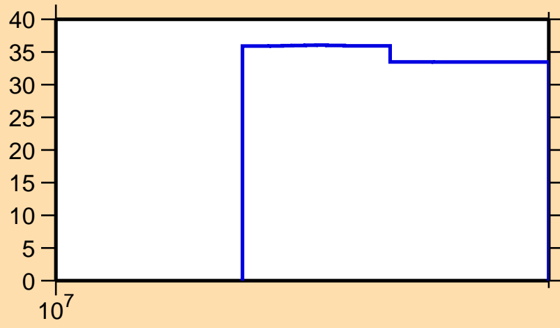
\Delta\sigma/\sigma vs. E for ^{57}\text{Cr}(n,\text{inel.})
