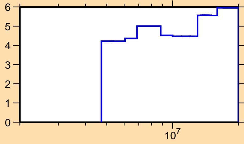
\Delta\sigma/\sigma vs. E for ^{57}\text{Cr}(n,n\text{onel.})
