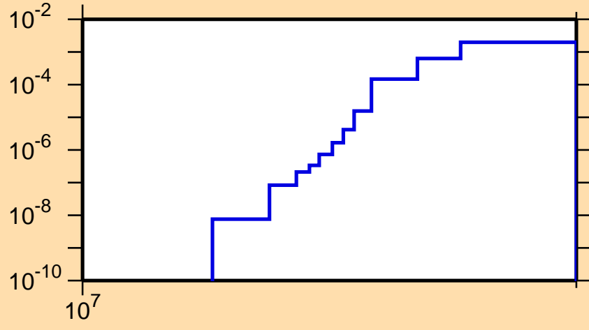
\sigma vs. E for ^{57}\text{Cr}(n,d)
