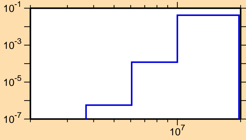
\sigma vs. E for ^{57}\text{Cr}(n,n\text{cont.})
