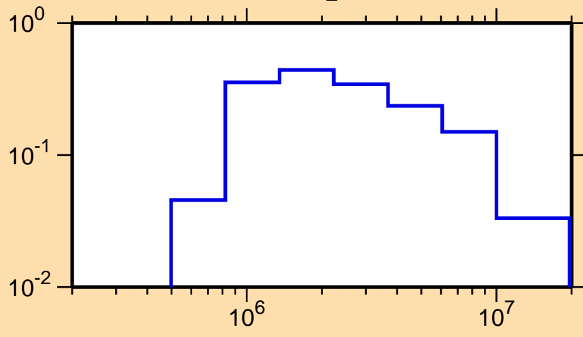
\sigma vs. E for ^{57}\text{Cr}(n,n_2)
