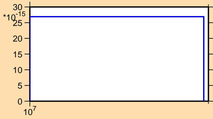
\sigma vs. E for ^{57}\text{Cr}(n,2np)
