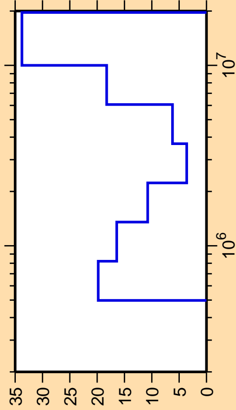
\Delta\sigma/\sigma vs. E for ^{57}\text{Cr}(n,n_2)
