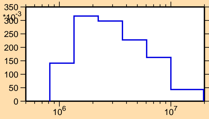
\sigma vs. E for ^{57}\text{Cr}(n,n_3)
