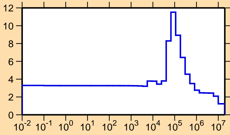
\sigma vs. E for ^{57}\text{Cr}(n,\text{el.})
