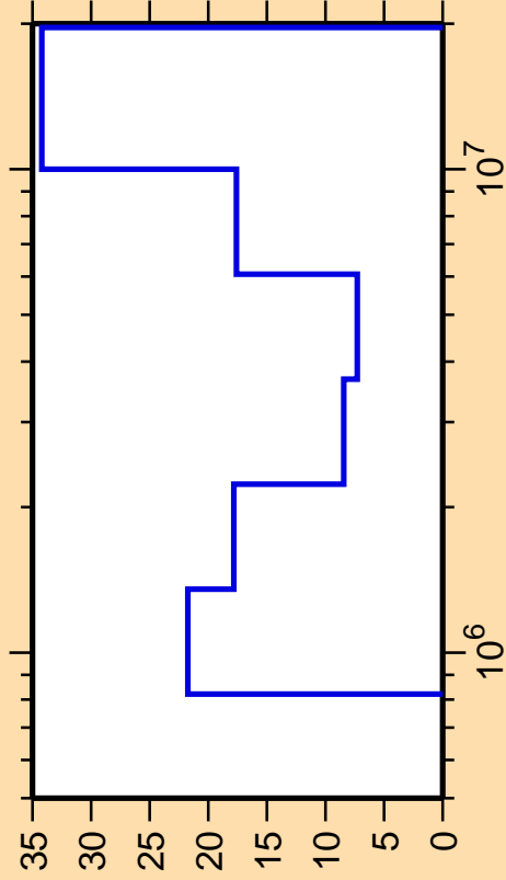
\Delta\sigma/\sigma vs. E for ^{57}\text{Cr}(n,n_3)
