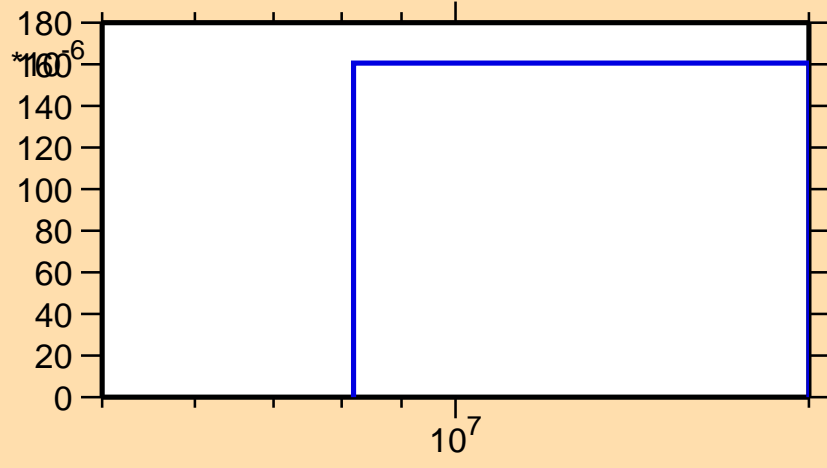
\sigma vs. E for ^{57}\text{Cr}(n,n\alpha)
