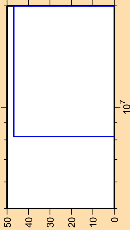
\Delta\sigma/\sigma vs. E for ^{57}\text{Cr}(n,\gamma)
