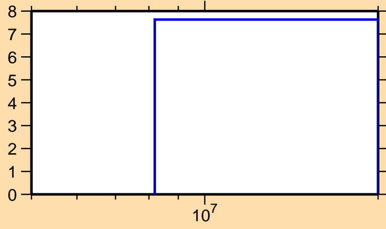
\Delta\sigma/\sigma vs. E for ^{57}\text{Cr}(n,2n)
