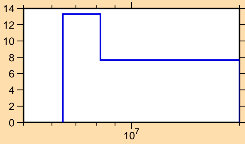
\Delta\sigma/\sigma vs. E for ^{57}\text{Cr}(n,el.)
