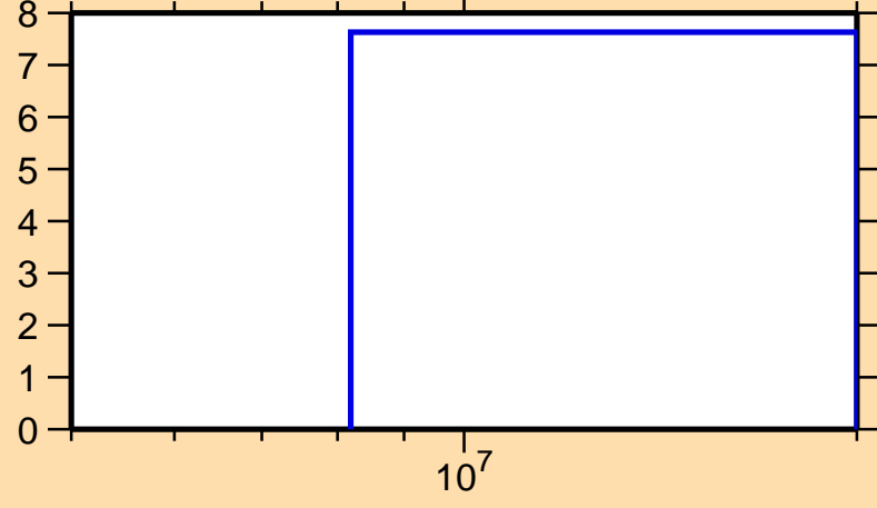
\Delta\sigma/\sigma vs. E for ^{57}\text{Cr}(n,2n)
