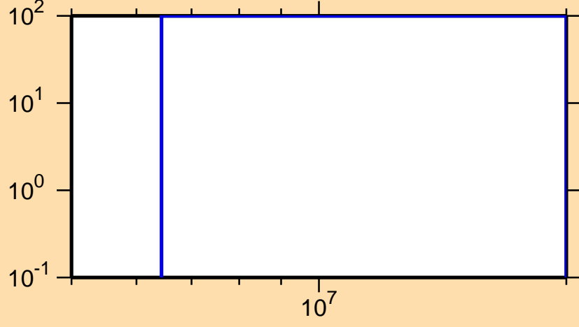
\Delta\sigma/\sigma vs. E for ^{57}\text{Cr}(n,ncont.)
