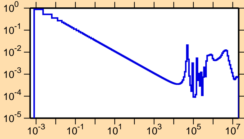
\sigma vs. E for ^{58}\text{Cr}(n,\gamma)
