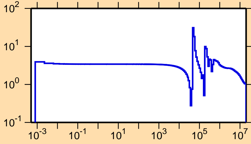
\sigma vs. E for ^{58}\text{Cr}(n,\text{el.})
