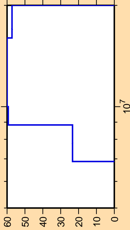
\Delta\sigma/\sigma vs. E for ^{58}\text{Cr}(n,n\text{cont.})
