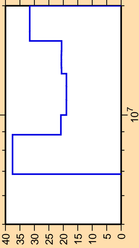
\Delta\sigma/\sigma vs. E for ^{58}\text{Cr}(n,2n)
