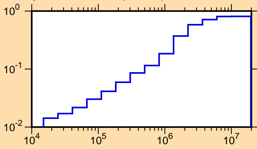
\mu vs. E for ^{59}\text{Cr}(\text{mt251})
