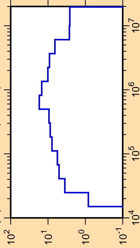
\Delta\mu/\mu vs. E for ^{59}\text{Cr}(\text{mt251})
