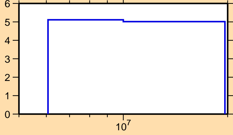
\Delta\sigma/\sigma vs. E for ^{59}\text{Cr}(n,\text{tot.})
