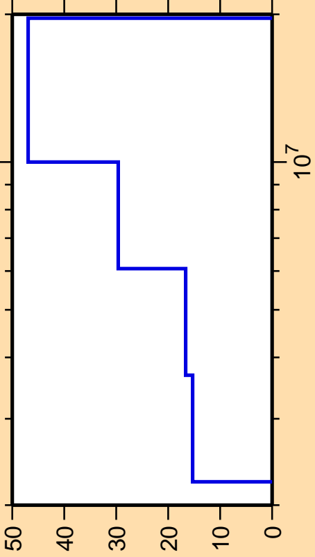
\Delta\sigma/\sigma vs. E for ^{59}\text{Cr}(n,n\text{cont.})
