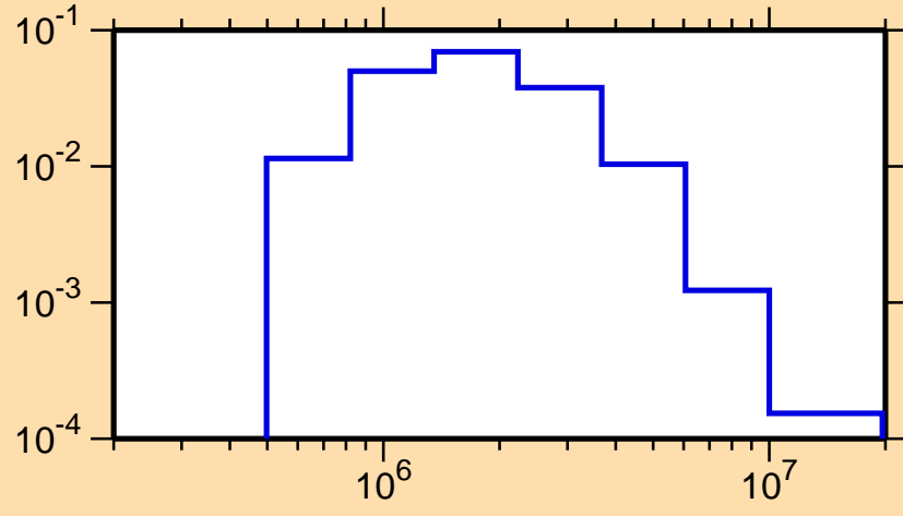
\sigma vs. E for ^{59}\text{Cr}(n,n_3)
