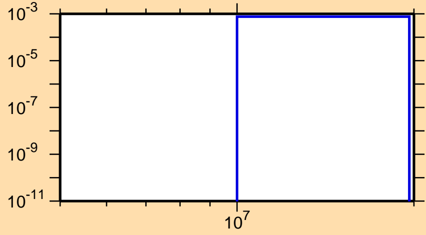
\sigma vs. E for ^{59}\text{Cr}(n,p)
