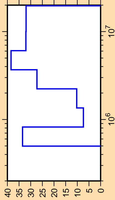
\Delta\sigma/\sigma vs. E for ^{59}\text{Cr}(n,n_3)
