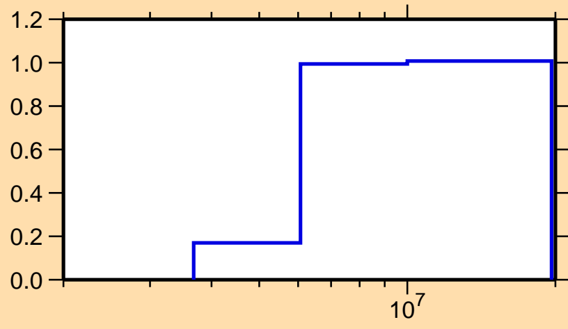
\sigma vs. E for ^{59}\text{Cr}(n,2n)
