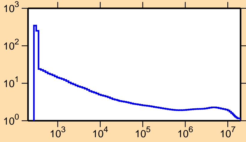
\sigma vs. E for ^{115}\text{Cs}(n,\text{nonel.})
