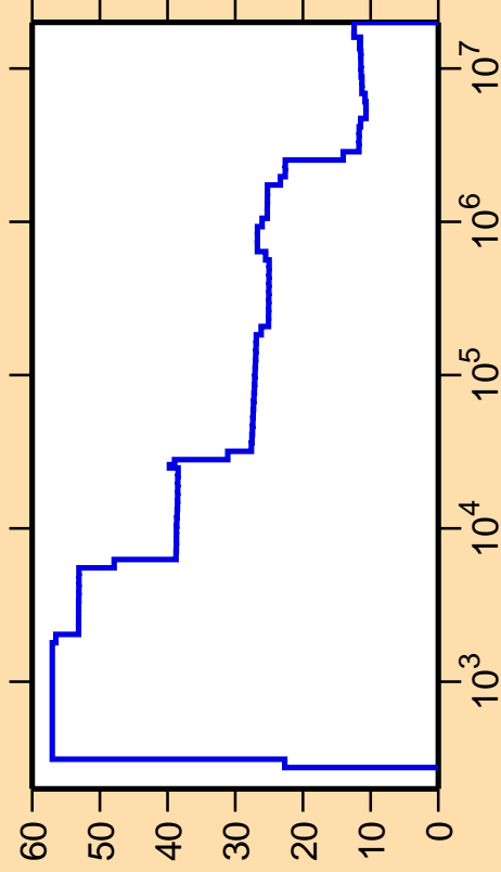
\Delta\sigma/\sigma vs. E for ^{115}\text{Cs}(n,\text{nonel.})
