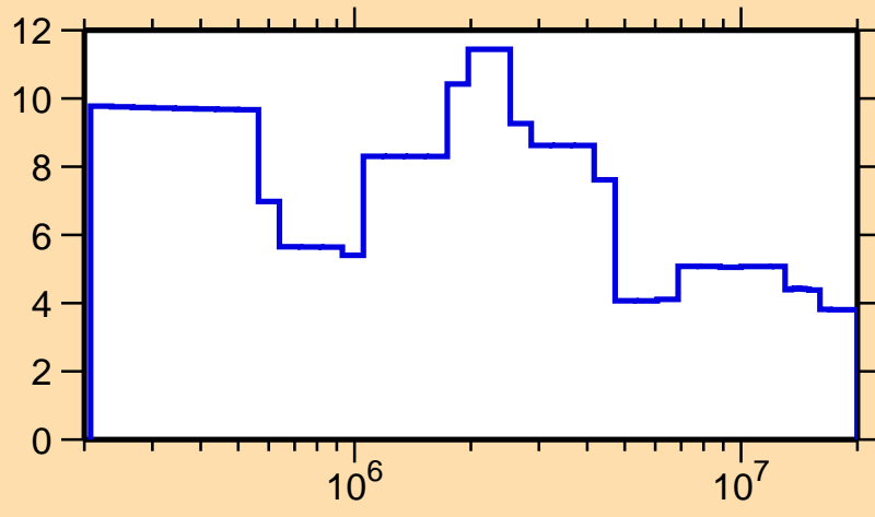
\Delta\sigma/\sigma vs. E for ^{115}\text{Cs}(n, tot.)
