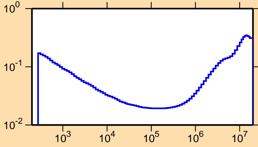
\sigma vs. E for ^{115}\text{Cs}(n,p\alpha)
