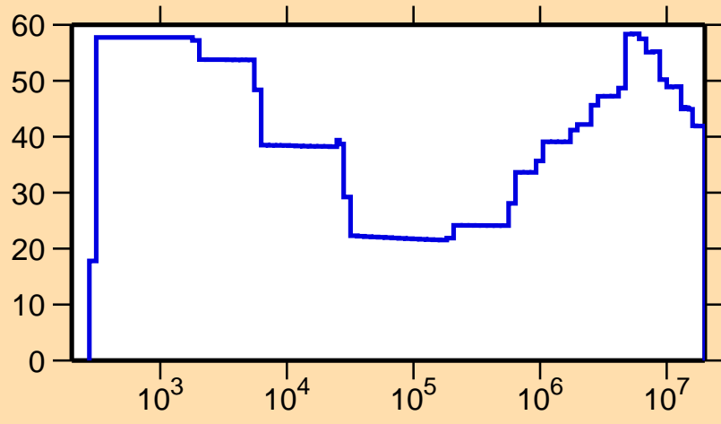
\Delta\sigma/\sigma vs. E for ^{115}\text{Cs}(n,p)
