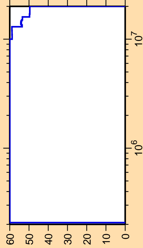
\Delta\sigma/\sigma vs. E for ^{115}\text{Cs}(n,\text{inel.})
