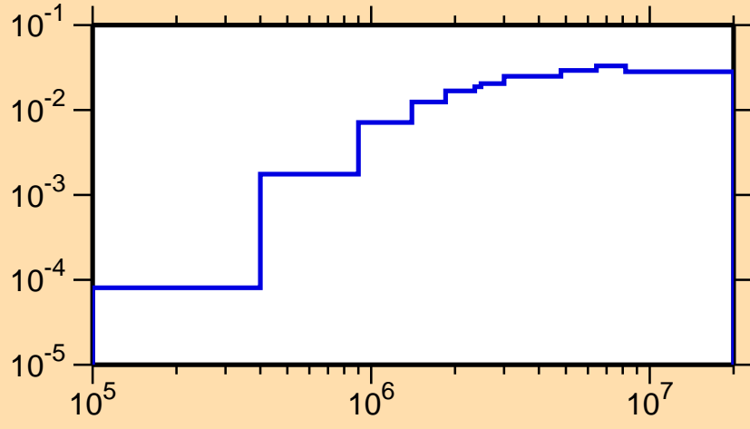
\sigma vs. E for ^{115}\text{Cs}(n,n\text{cont.})
