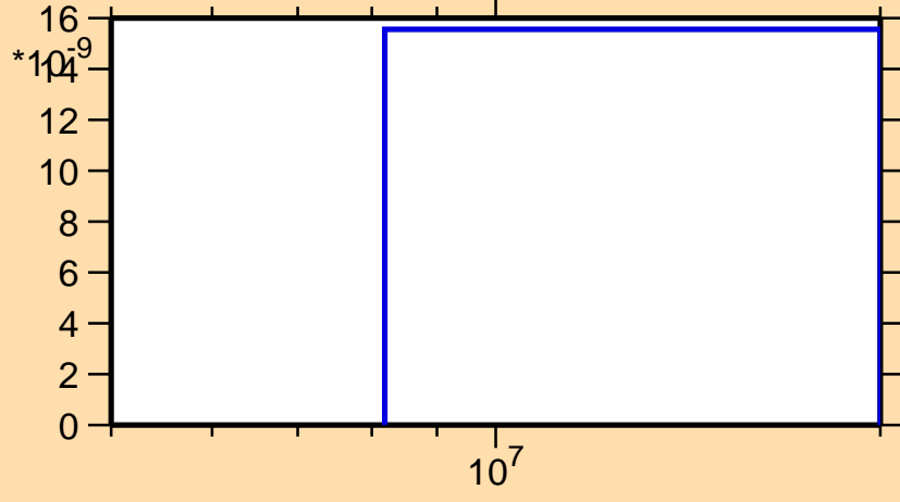
\sigma vs. E for ^{115}\text{Cs}(n,nd)
