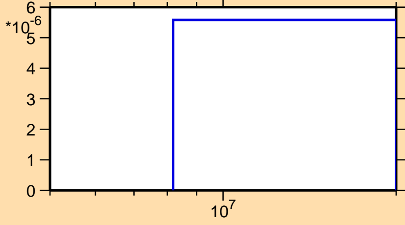
\sigma vs. E for ^{115}\text{Cs}(n,pt)
