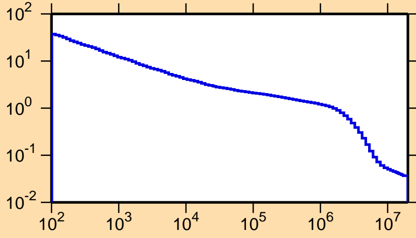
\sigma vs. E for ^{116}\text{Cs}(n,p)
