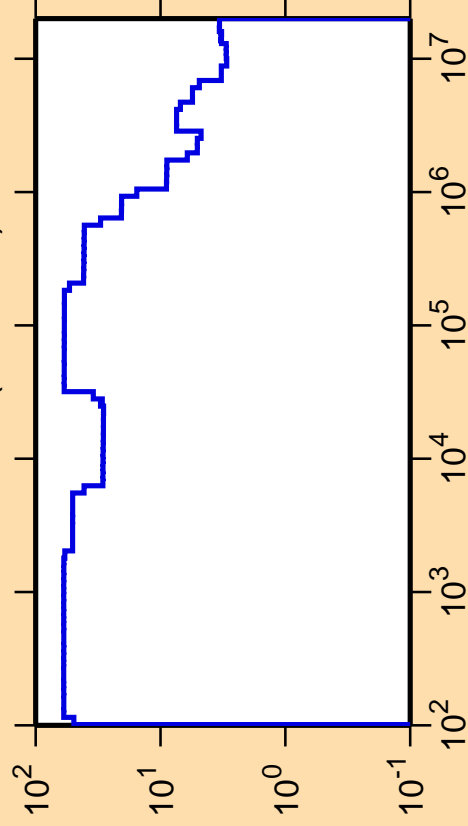
\Delta\sigma/\sigma vs. E for ^{116}\text{Cs}(n,\text{nonel.})
