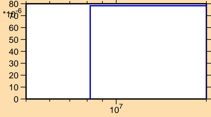
\sigma vs. E for ^{116}\text{Cs}(n,2np)
