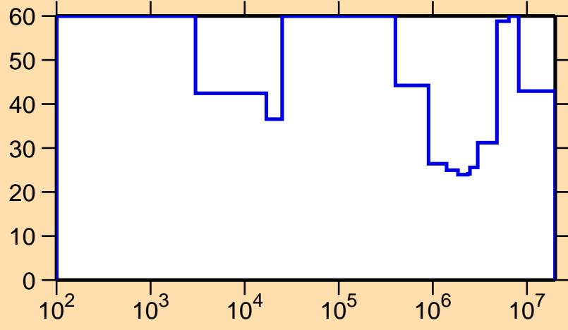
\Delta\sigma/\sigma vs. E for ^{116}\text{Cs}(n,p)
