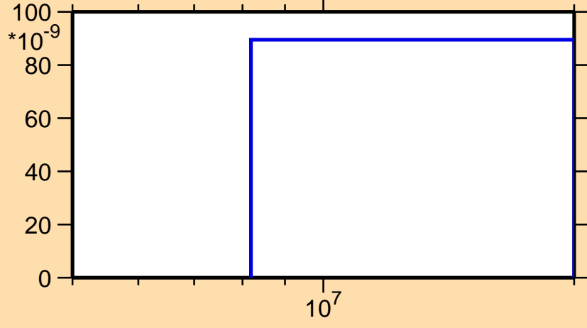
\sigma vs. E for ^{116}\text{Cs}(n,2n\alpha)
