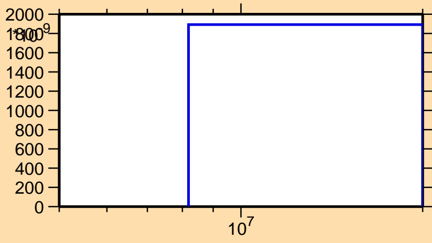
\sigma vs. E for ^{116}\text{Cs}(n,\text{nd})
