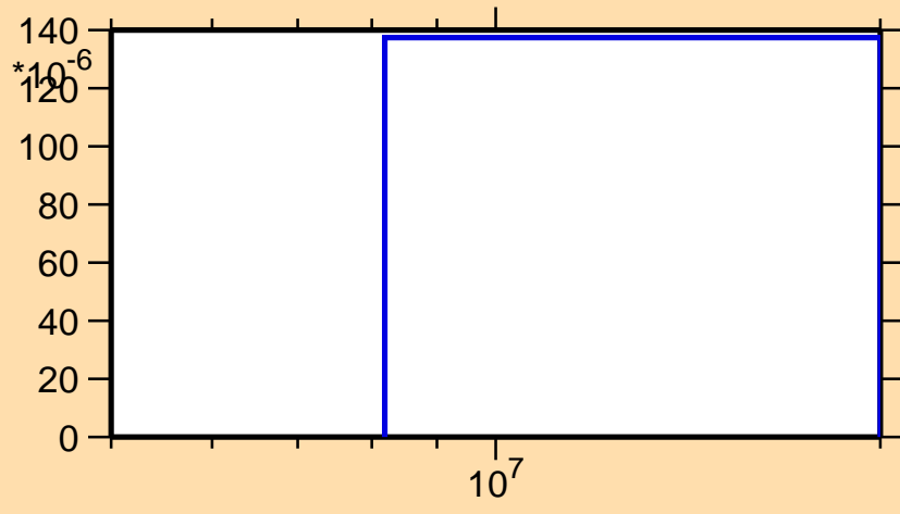
\sigma vs. E for ^{116}\text{Cs}(n,\text{pt})
