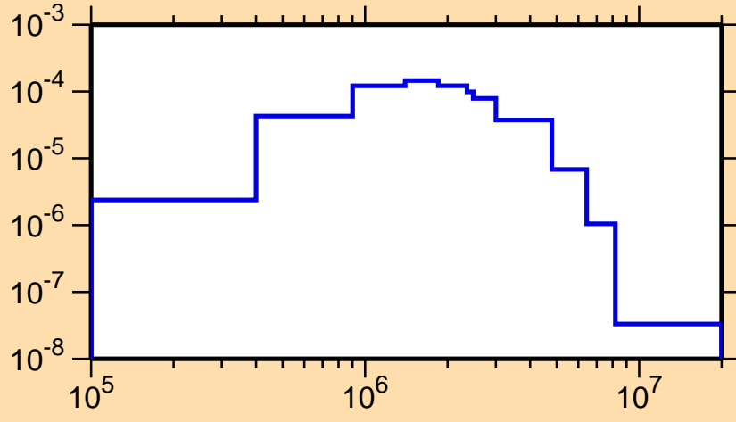
\sigma vs. E for ^{116}\text{Cs}(n,n_2)
