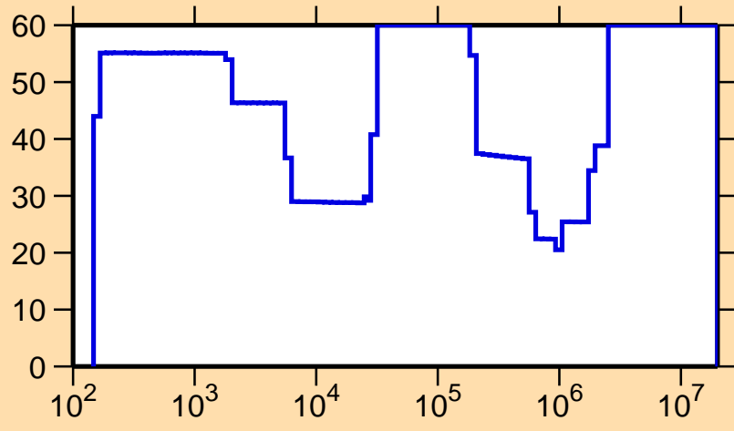
\Delta\sigma/\sigma vs. E for ^{117}\text{Cs}(n,p)
