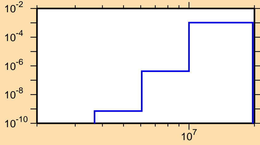
\sigma vs. E for ^{117}\text{Cs}(n,\text{He}3)
