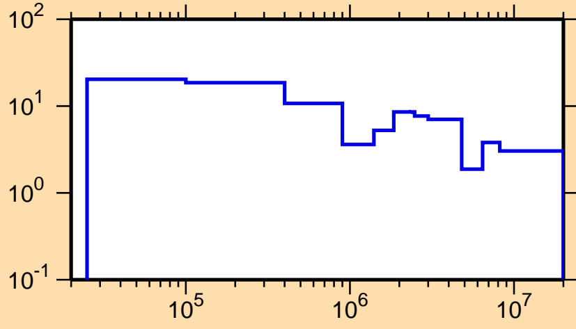
\Delta\sigma/\sigma vs. E for ^{117}\text{Cs}(n, tot.)
