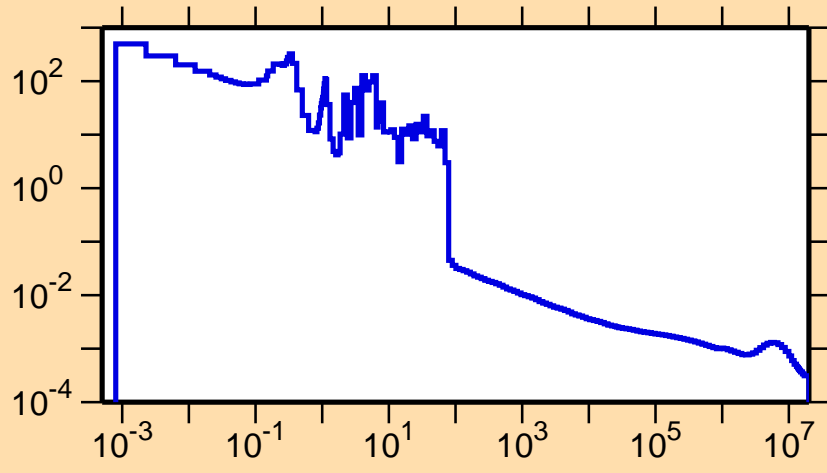
\sigma vs. E for ^{118}\text{Cs}(n,\gamma)
