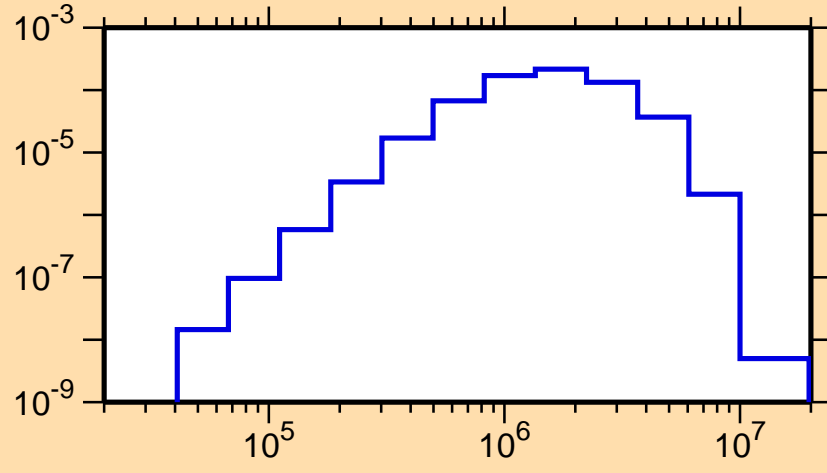
\sigma vs. E for ^{118}\text{Cs}(n,n_2)
