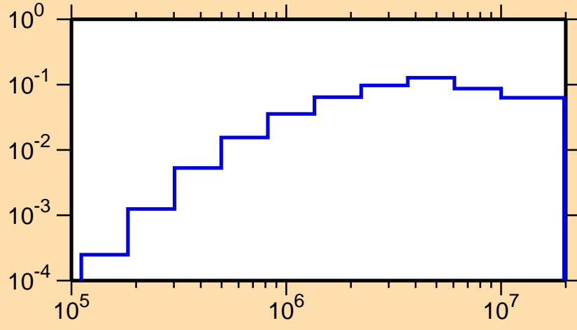
\sigma vs. E for ^{118}\text{Cs}(n,n\text{cont.})
