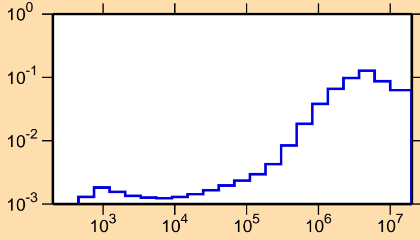
\sigma vs. E for ^{118}\text{Cs}(n,\text{inel.})
