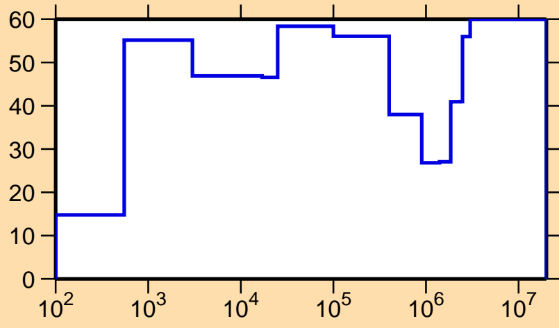
\Delta\sigma/\sigma vs. E for ^{118}\text{Cs}(n,p)
