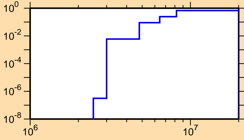
\sigma vs. E for ^{118}\text{Cs}(n,np)
