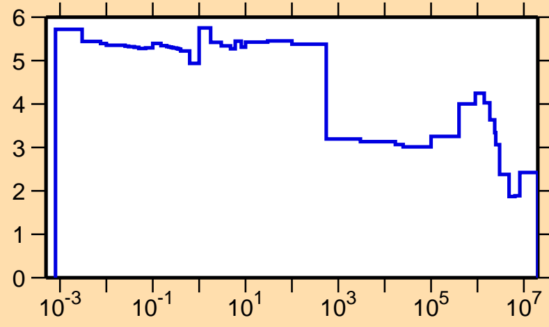
\sigma vs. E for ^{118}\text{Cs}(n,\text{el.})
