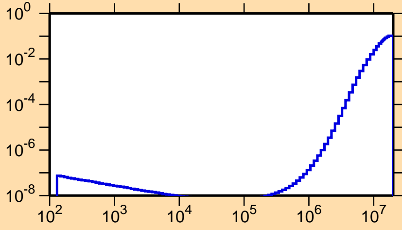
\sigma vs. E for ^{119}\text{Cs}(n,p\alpha)
