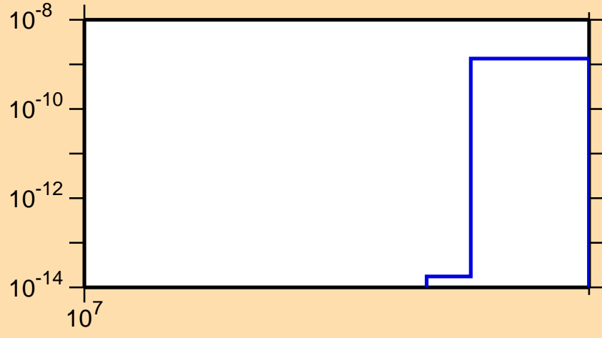
\sigma vs. E for ^{119}\text{Cs}(n,nt)
