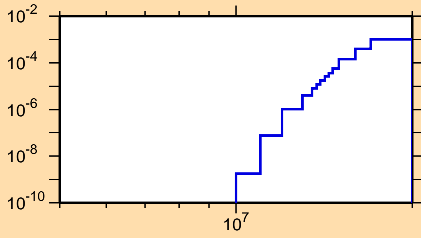
\sigma vs. E for ^{119}\text{Cs}(n,\text{pd})
