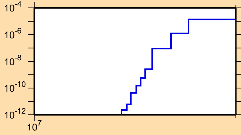
\sigma vs. E for ^{119}\text{Cs}(n,\text{nd})
