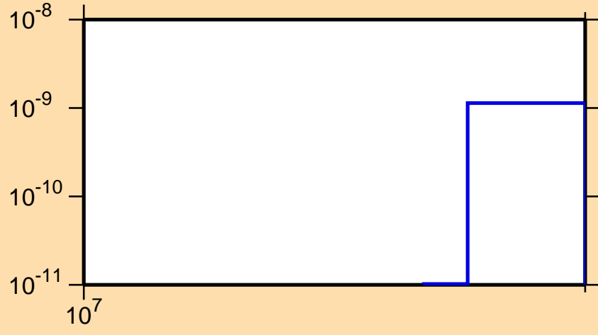
\sigma vs. E for ^{119}\text{Cs} (mt 34)
