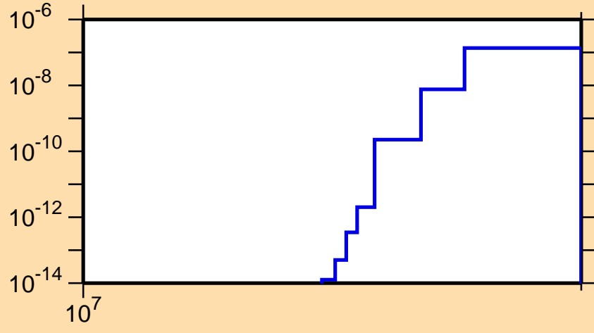
\sigma vs. E for ^{119}\text{Cs}(n,2n\alpha)
