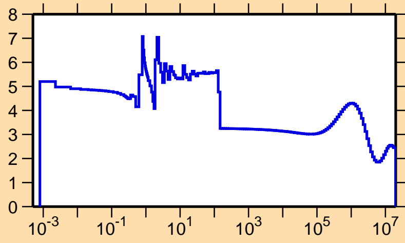
\sigma vs. E for ^{119}\text{Cs}(n,\text{el.})
