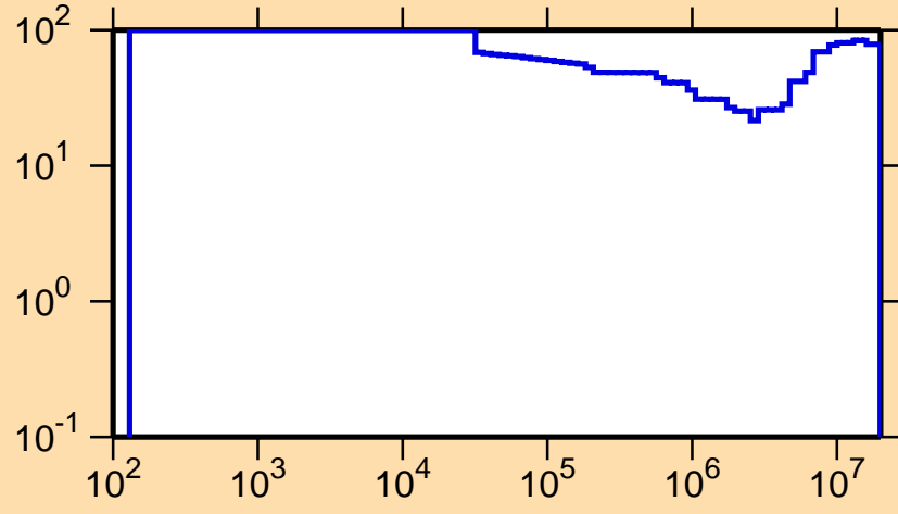
\Delta\sigma/\sigma vs. E for ^{119}\text{Cs}(n,p)
