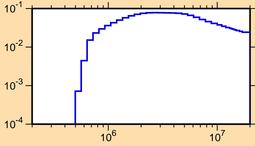
\sigma vs. E for ^{119}\text{Cs}(n,n_3)
