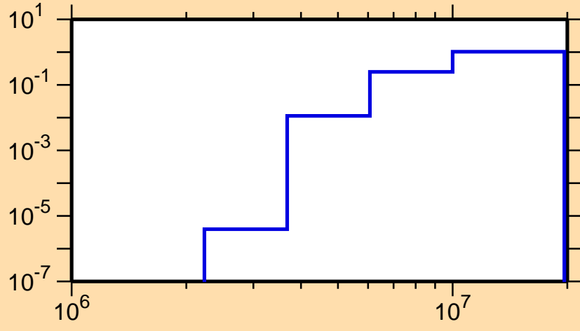
\sigma vs. E for ^{119}\text{Cs}(n,np)
