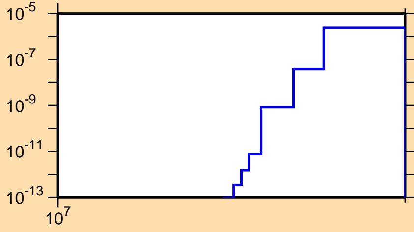
\sigma vs. E for ^{119}\text{Cs}(n,pt)
