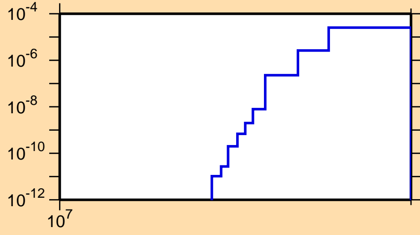
\sigma vs. E for ^{119}\text{Cs}(n,nd)
