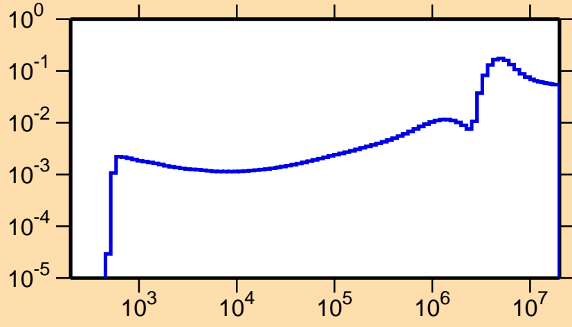
\sigma vs. E for ^{119}\text{Cs}(n,\text{inel.})
