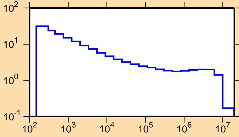
\sigma vs. E for ^{119}\text{Cs}(n,p)
