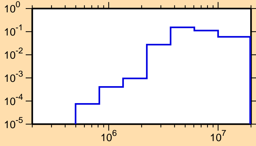
\sigma vs. E for ^{119}\text{Cs}(n,n\text{cont.})
