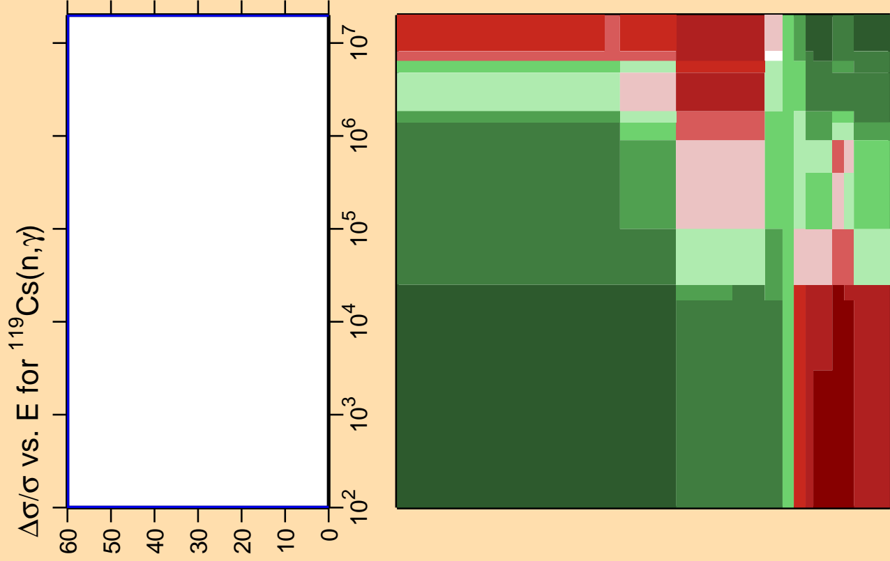
Correlation Matrix
