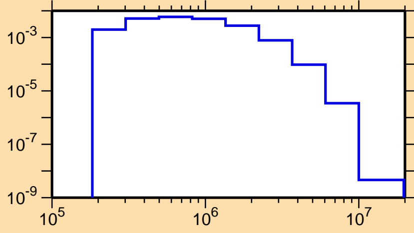
\sigma vs. E for ^{120}\text{Cs}(n,n_4)
