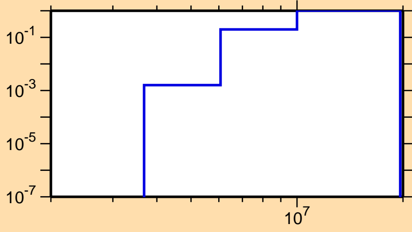
\sigma vs. E for ^{120}\text{Cs}(n,np)
