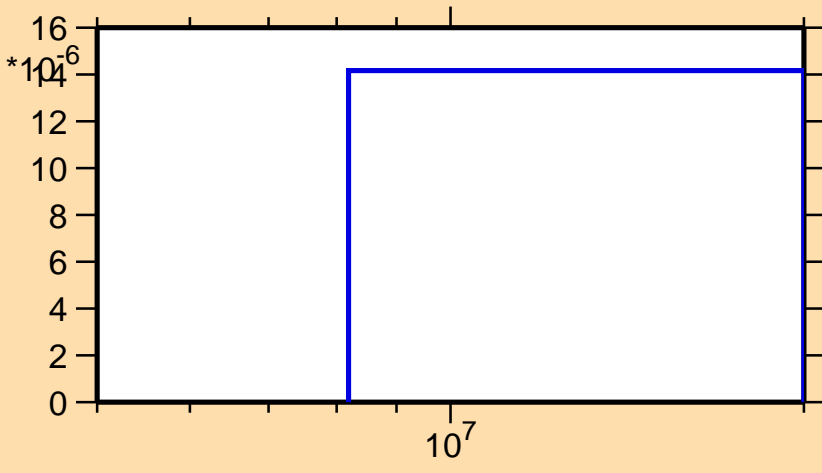
\sigma vs. E for ^{120}\text{Cs}(n,nd)
