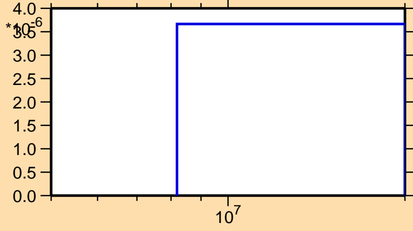
\sigma vs. E for ^{120}\text{Cs}(n,\text{pd})
