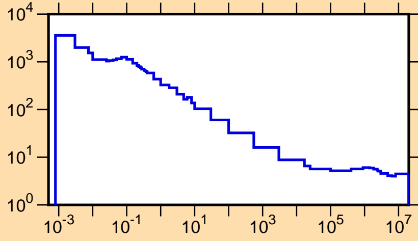
\sigma vs. E for ^{120}\text{Cs}(n,\text{tot.})
