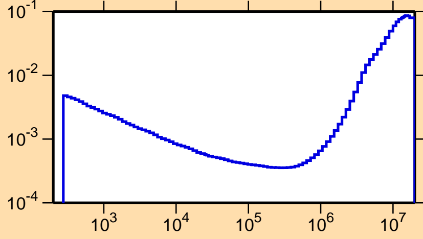
\sigma vs. E for ^{121}\text{Cs}(n,\alpha)
