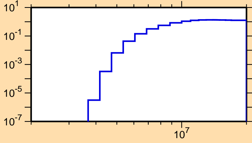
\sigma vs. E for ^{121}\text{Cs}(n,np)
