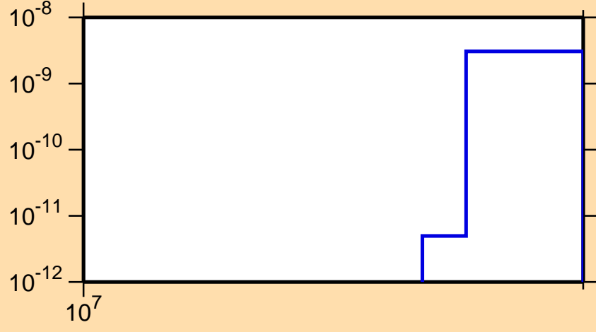
\sigma vs. E for ^{121}\text{Cs}(n,pt)
