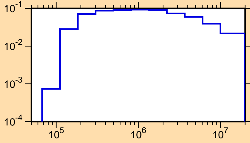
\sigma vs. E for ^{121}\text{Cs}(n,n_3)
