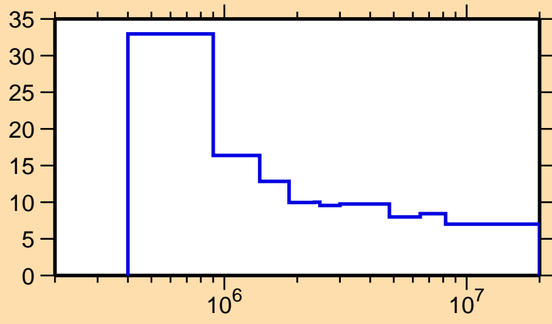
\Delta\sigma/\sigma vs. E for ^{121}\text{Cs}(n,\text{nonel.})
