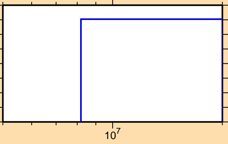
\sigma vs. E for ^{121}\text{Cs}(n,2np)
