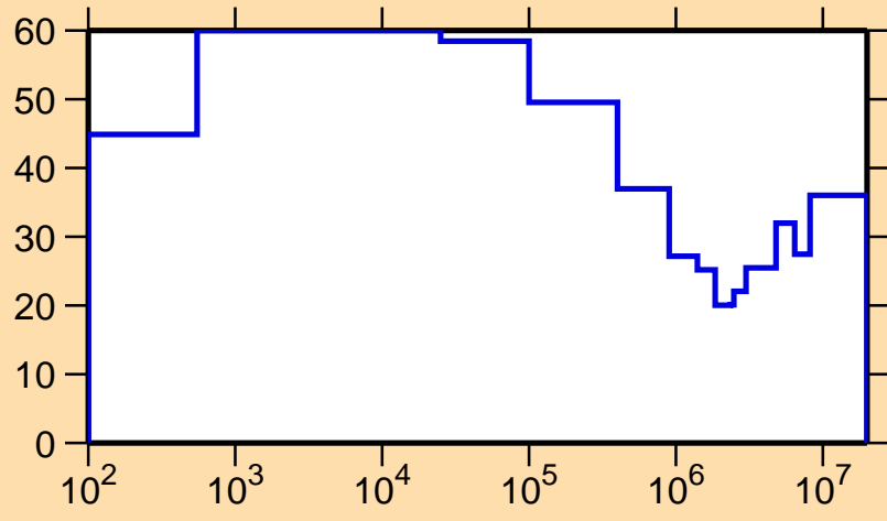
\Delta\sigma/\sigma vs. E for ^{121}\text{Cs}(n,p)
