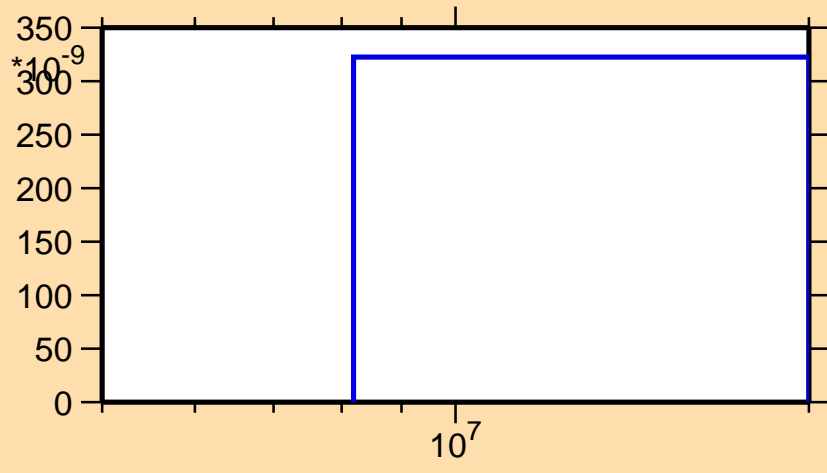
\sigma vs. E for ^{121}\text{Cs}(n,nd)
