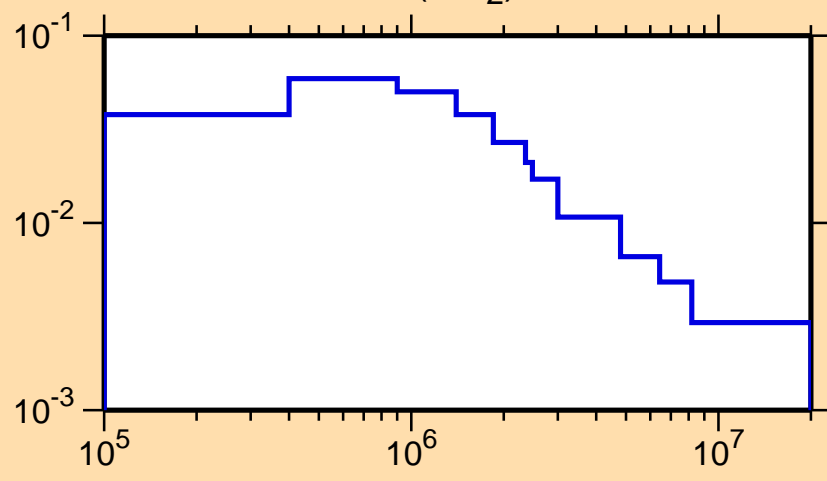
\sigma vs. E for ^{121}\text{Cs}(n,n_2)
