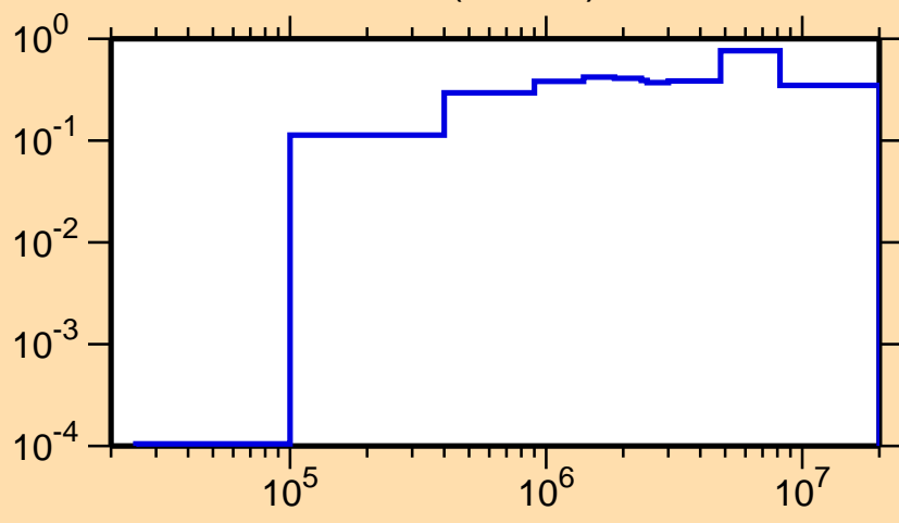
\sigma vs. E for ^{121}\text{Cs}(n,\text{inel.})
