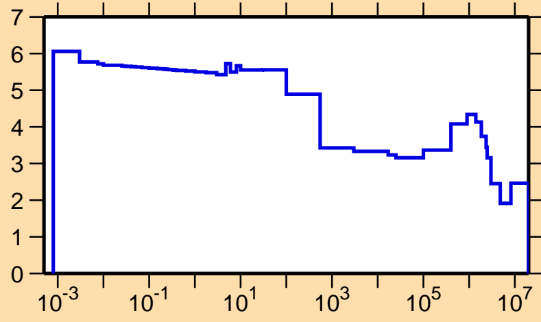
\sigma vs. E for ^{121}\text{Cs}(n,\text{el.})
