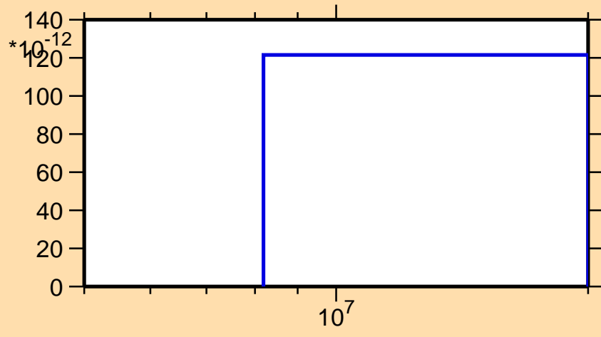
\sigma vs. E for ^{121}\text{Cs}(n,nt)
