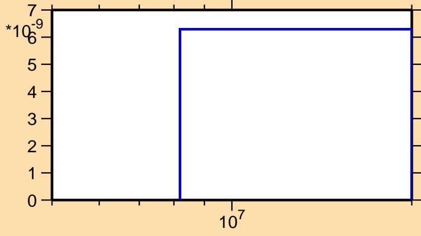
\sigma vs. E for ^{121}\text{Cs}(n,2n\alpha)
