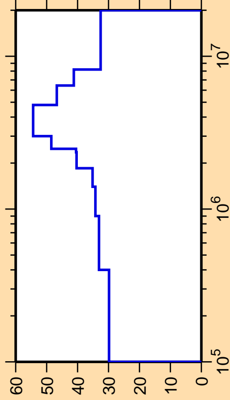
\Delta\sigma/\sigma vs. E for ^{121}\text{Cs}(n,n_2)
