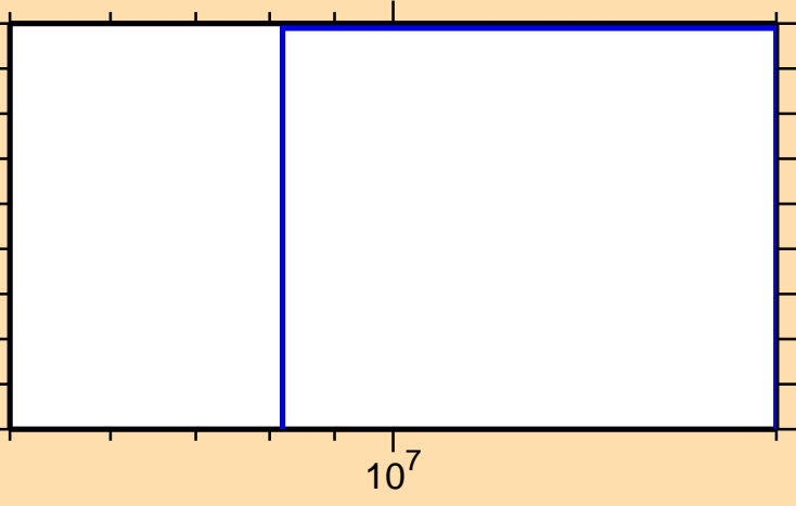
\sigma vs. E for ^{121}\text{Cs} (mt 34)
