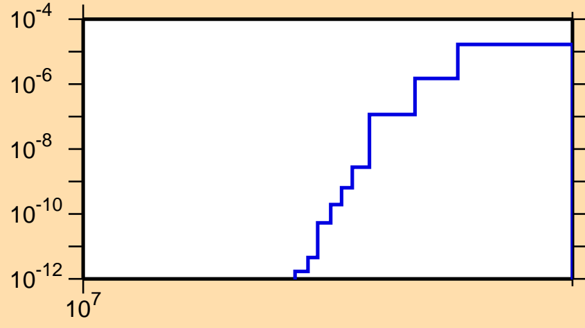
\sigma vs. E for ^{121}\text{Cs}(n,nd)
