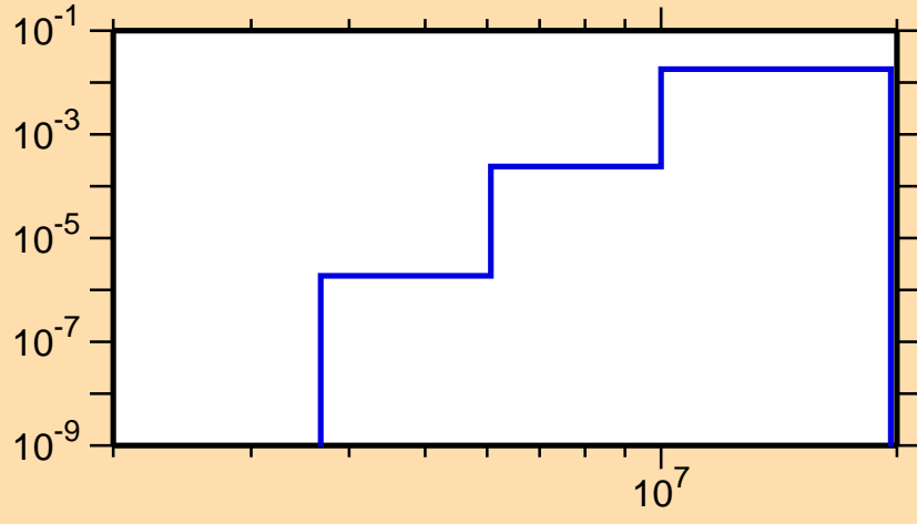
\sigma vs. E for ^{121}\text{Cs}(n,n\alpha)
