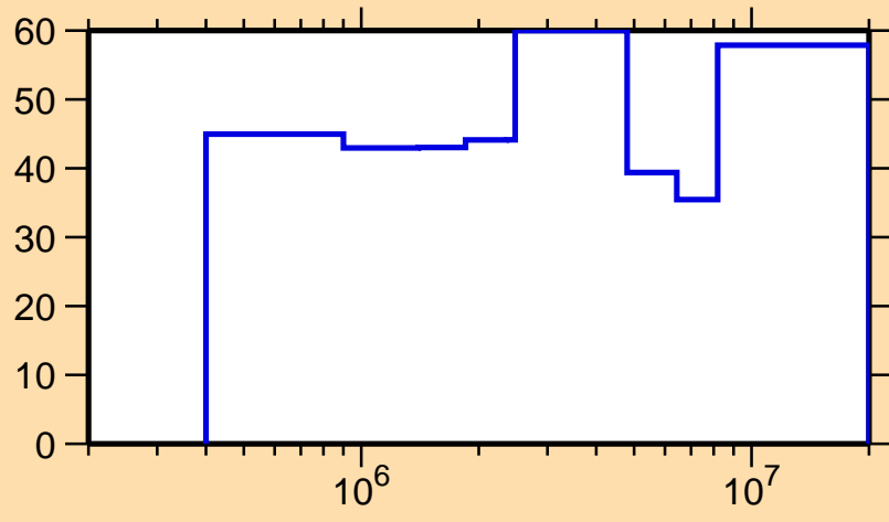
\Delta\sigma/\sigma vs. E for ^{121}\text{Cs}(n,n\text{cont.})
