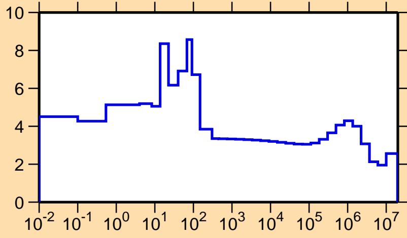
\sigma vs. E for ^{122}\text{Cs}(n,\text{el.})
