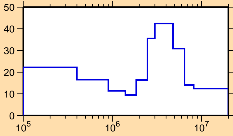
\Delta\sigma/\sigma vs. E for ^{122}\text{Cs}(n, el.)
