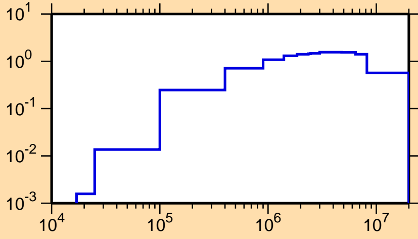
\sigma vs. E for ^{122}\text{Cs}(n,\text{inel.})
