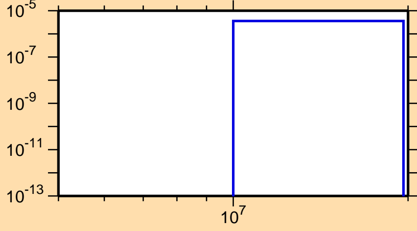
\sigma vs. E for ^{122}\text{Cs}(n,nd)
