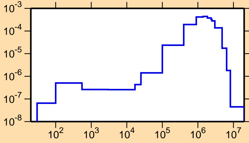
\sigma vs. E for ^{122}\text{Cs}(n,n_2)
