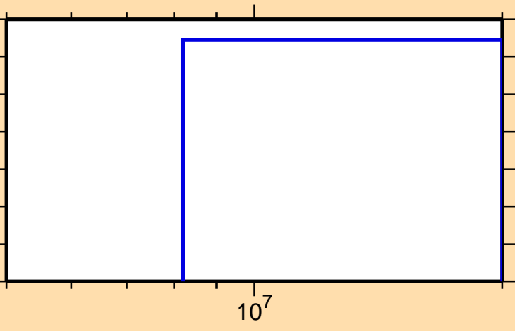
\sigma vs. E for ^{123}\text{Cs}(n,2np)
