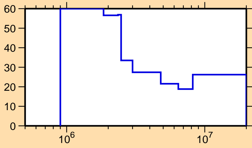
\Delta\sigma/\sigma vs. E for ^{123}\text{Cs}(n,n\text{cont.})
