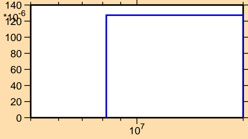
\sigma vs. E for ^{123}\text{Cs}(n,t)
