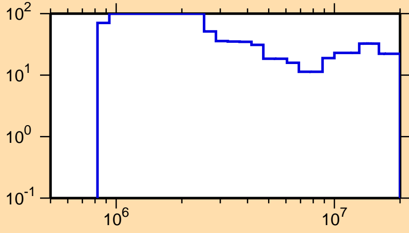
\Delta\sigma/\sigma vs. E for ^{123}\text{Cs}(n,n\text{cont.})
