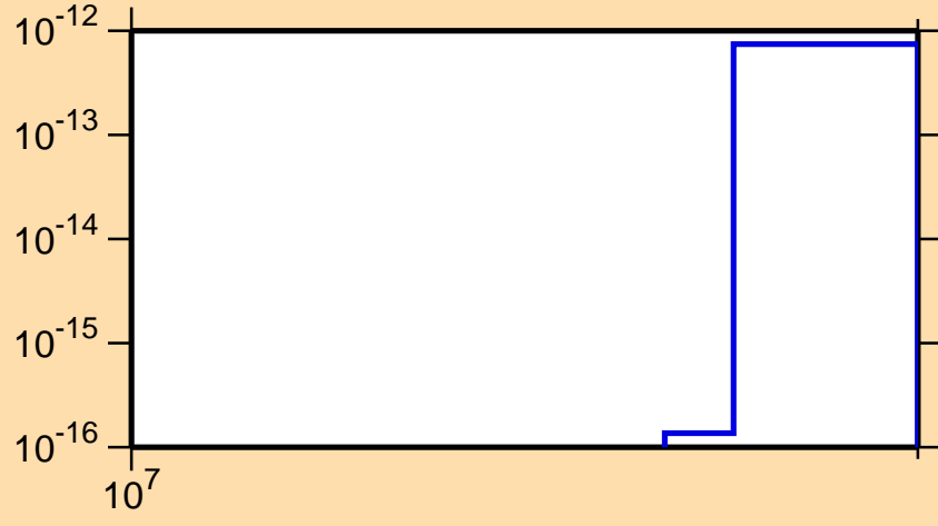
\sigma vs. E for ^{123}\text{Cs} (mt 34)
