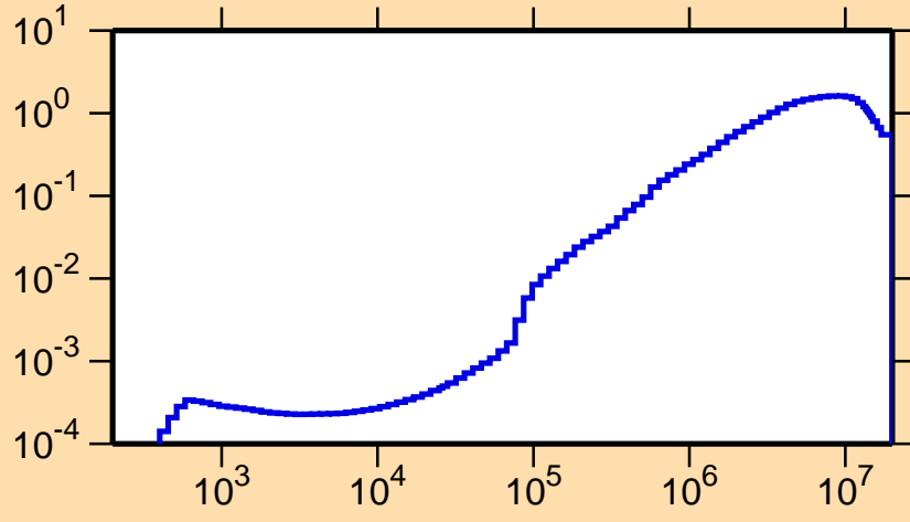
\sigma vs. E for ^{123}\text{Cs}(n,\text{inel.})
