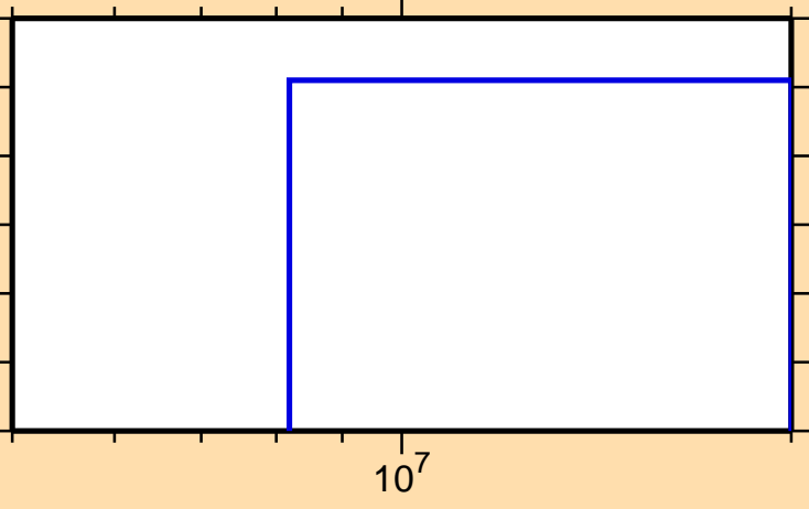
\sigma vs. E for ^{123}\text{Cs}(\text{mt117})
