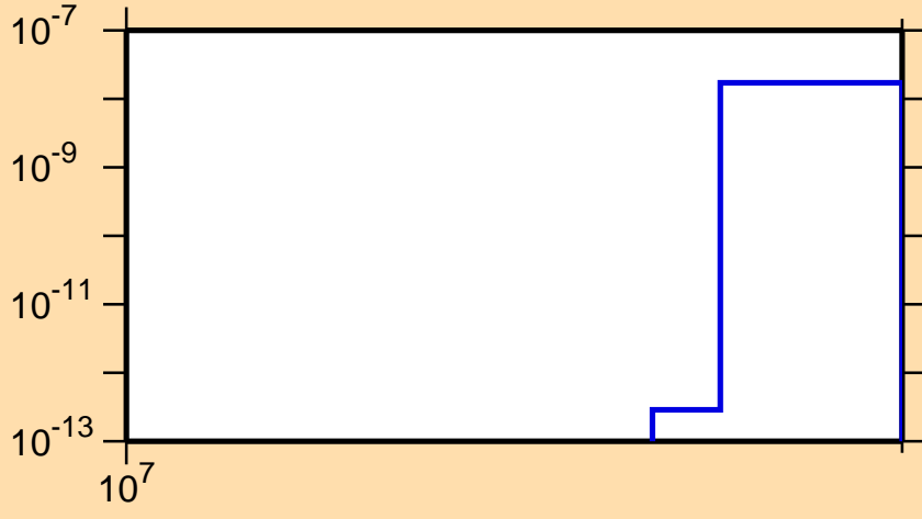
\sigma vs. E for ^{124}\text{Cs}(n,nt)
