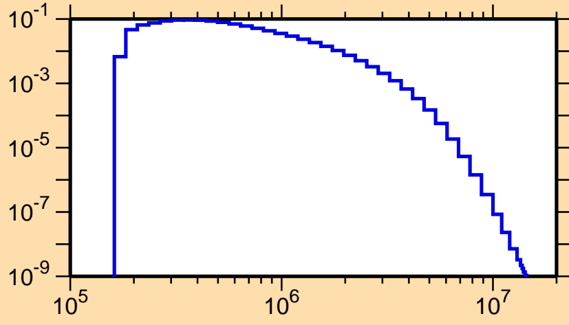
\sigma vs. E for ^{124}\text{Cs}(n,n_1)
