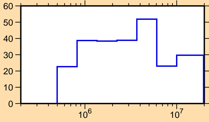
\Delta\sigma/\sigma vs. E for ^{124}\text{Cs}(n, el.)
