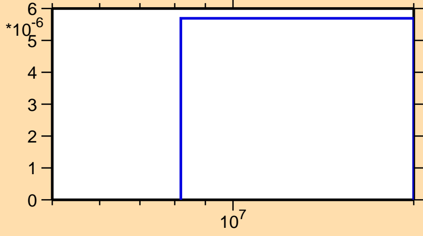
\sigma vs. E for ^{124}\text{Cs}(n,nd)
