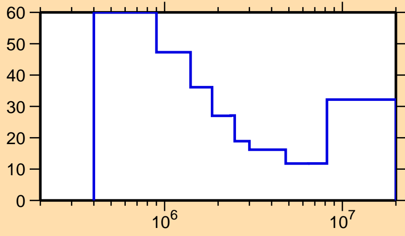
\Delta\sigma/\sigma vs. E for ^{124}\text{Cs}(n,n\text{cont.})
