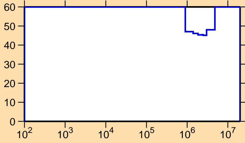
\Delta\sigma/\sigma vs. E for ^{124}\text{Cs}(n,p)
