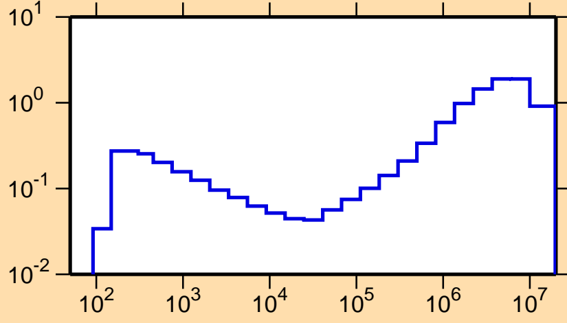
\sigma vs. E for ^{124}\text{Cs}(n,\text{inel.})
